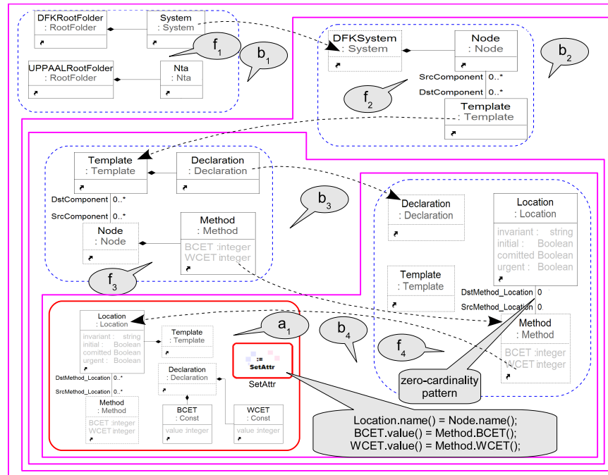
Figure 3: Example PML Block hierarchy
