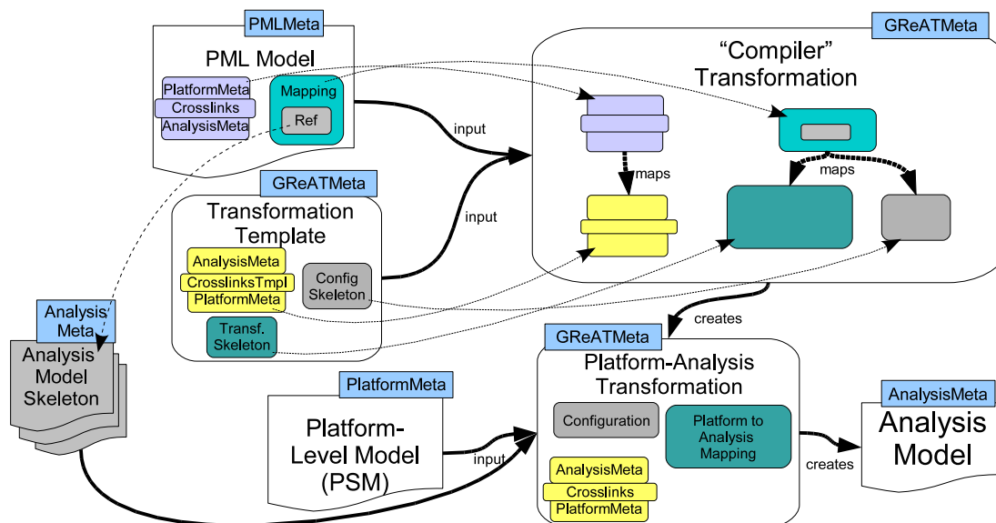
Figure 4: High-level overview of the PML→GReAT transformation
