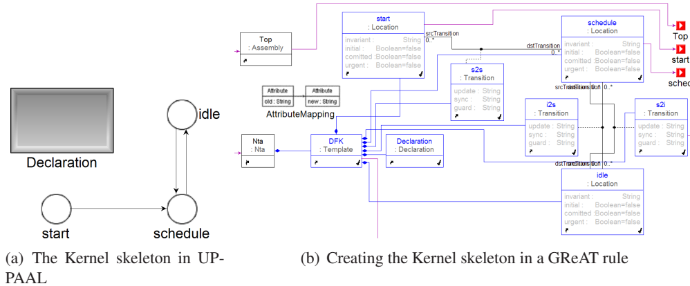
Figure 1: Creating an analysis model fragment in GREAT
