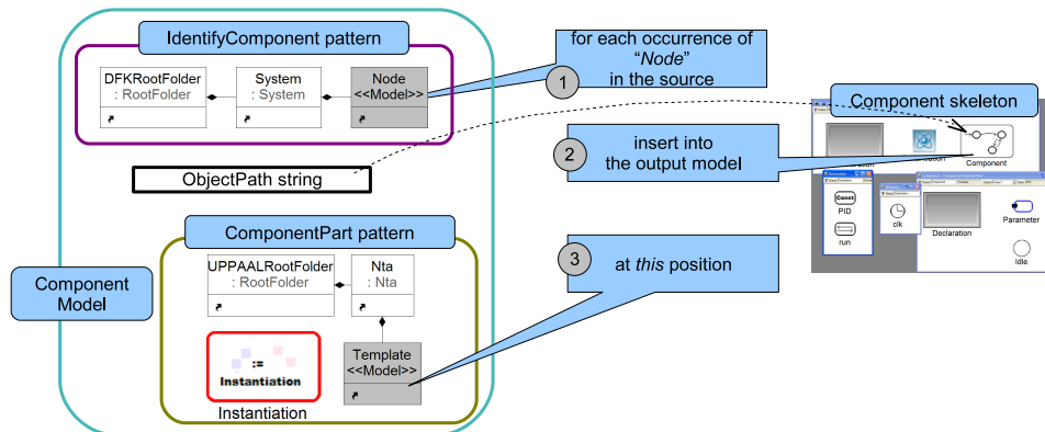
Figure 2: Visualization of the ComponentModel concept
