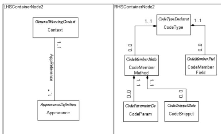
Figure 6: The rule MatchAppearances
