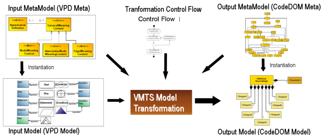
Figure 4: Model Transformation in VMTS - Overview
