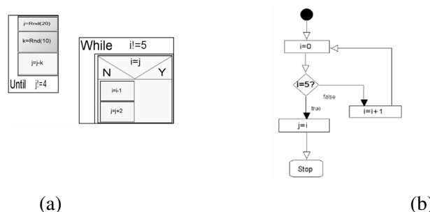
Figure 7: Example plug-ins - (a) Nassie-Schneidermann (b) Flowchart
