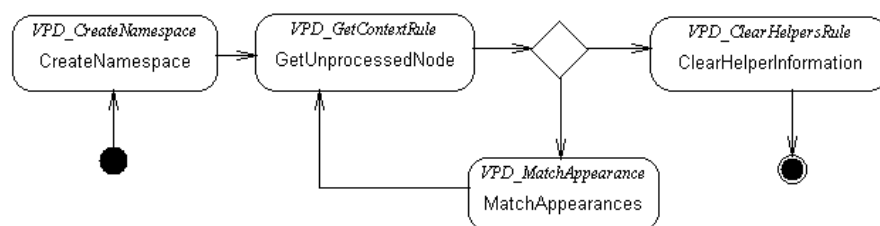
Figure 5: VMTS Presentation DSL - Control Flow
