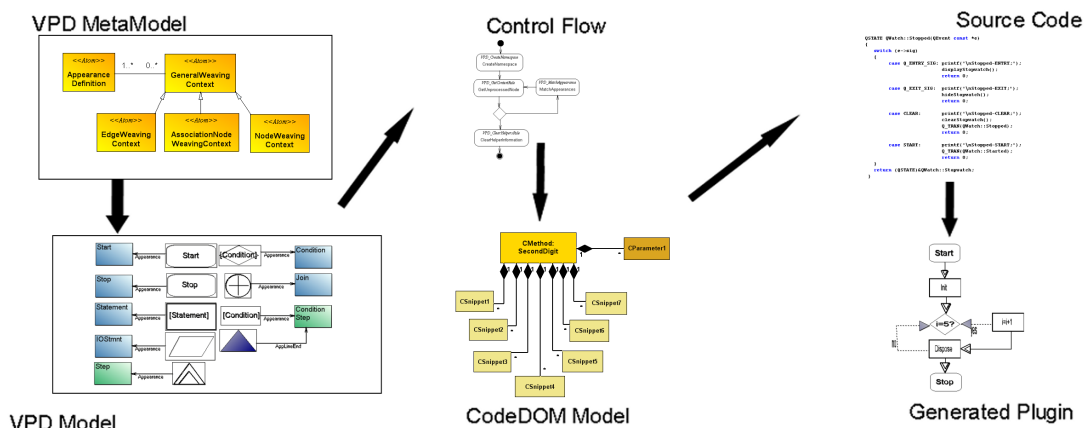
Figure 1: Concrete Syntax Definition - Overview
