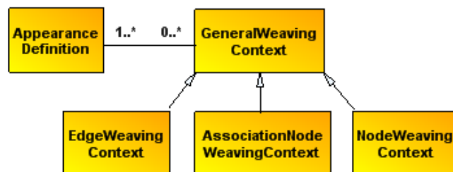
Figure 3: VMTS Presentation DSL - Metamodel
