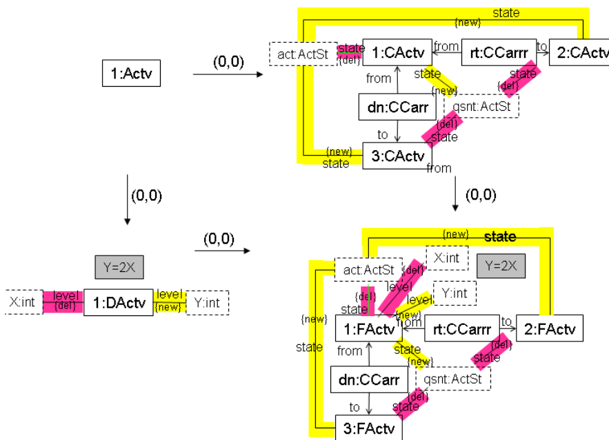
Figure 12: The resulting rule specifying the condition of application.
