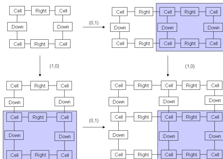
Figure 3: The pushout construction for grids
